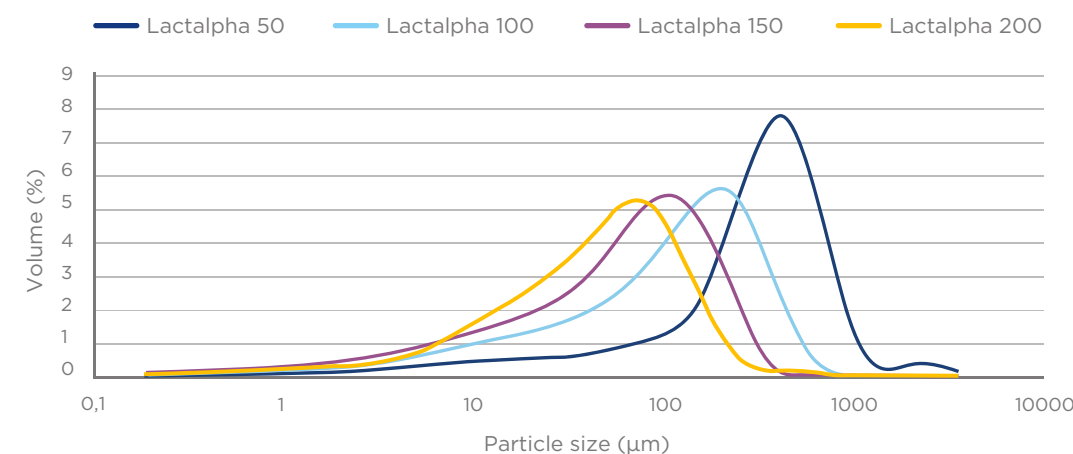
PSD by laser diffraction (indicative values)
